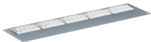
Cover plate with cable entry flange 1350x600 (WxD)
